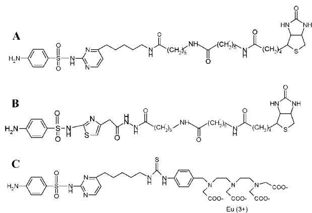
Figure 3. Sulfonamide derivatives synthesized for use in phage display and immunoassays: (A) biotinylated sulfamerazine derivative; (B) biotinylated sulfathiazole derivative; (C) N1-europium chelate labeled sulfamerazine derivative.
