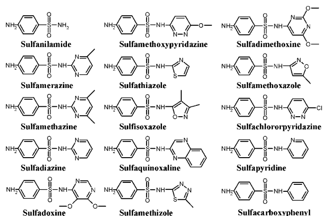
Figure 1. Structures of selected sulfonamides.
